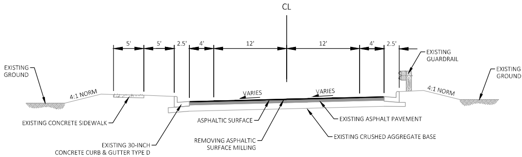
FINISHED URBAN SECTION TAINTER LAKE BRIDGE
