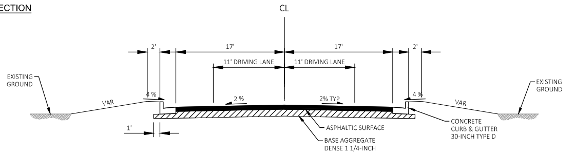
FINISHED URBAN TYPICAL SECTION
