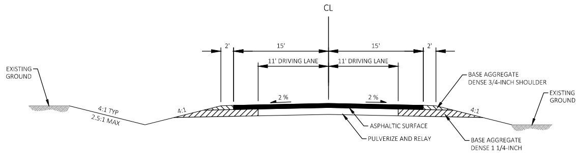
FINISHED RURAL TYPICAL SECTION
